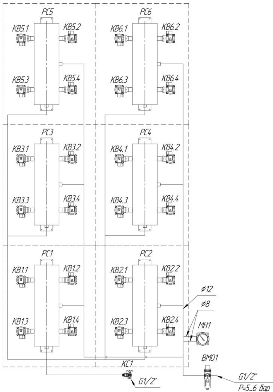
Рис. 57 FCS-ECO-24-H
