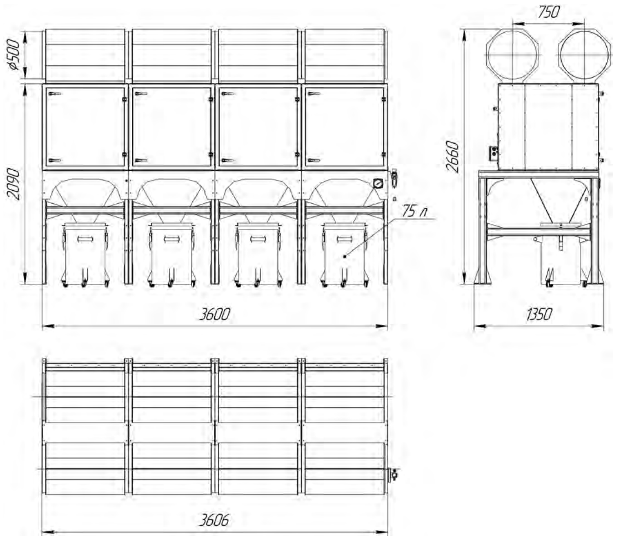
Рис. 30 FCS-ECO-16-L
