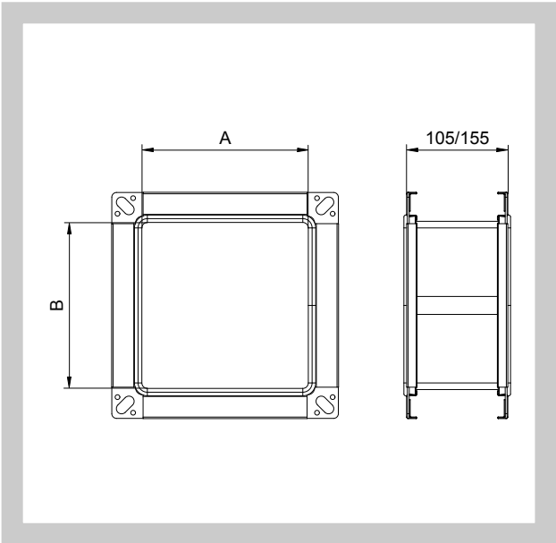
Fig. 2 Damping pad - Square
