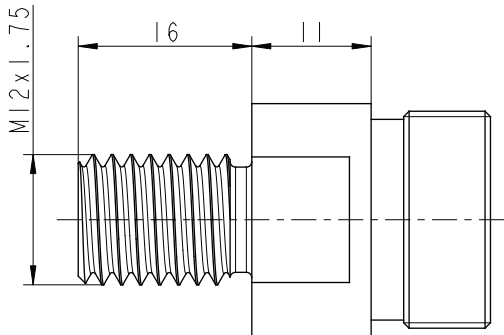
Option "M" Piston 0231094, Stainless steel AISI 304
