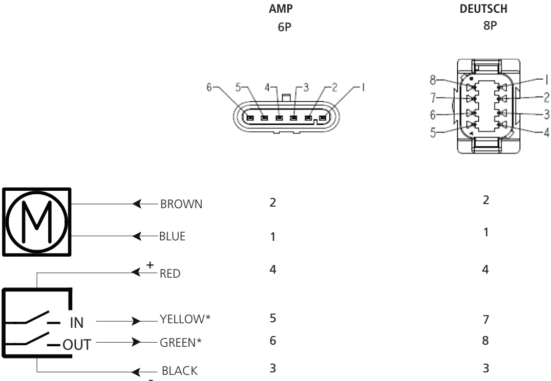
Standard connector front view
