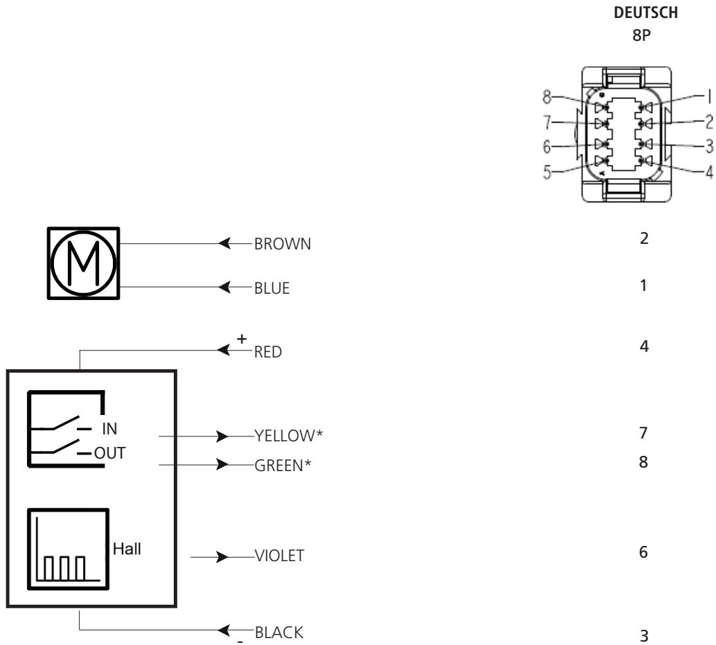
Standard connector front view
