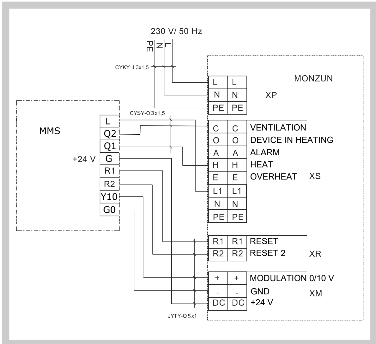
Fig. 19 Connection diagram of the MONZUN-CP heater with control box MMS
