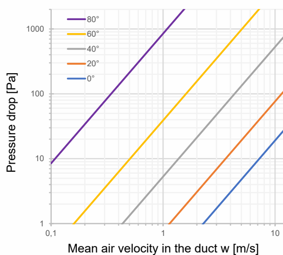
Graph 2 Pressure drop as function of the air velocity and blade angle, damper in the duct
