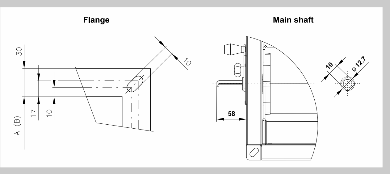
Fig. 6 Connection dimensions
