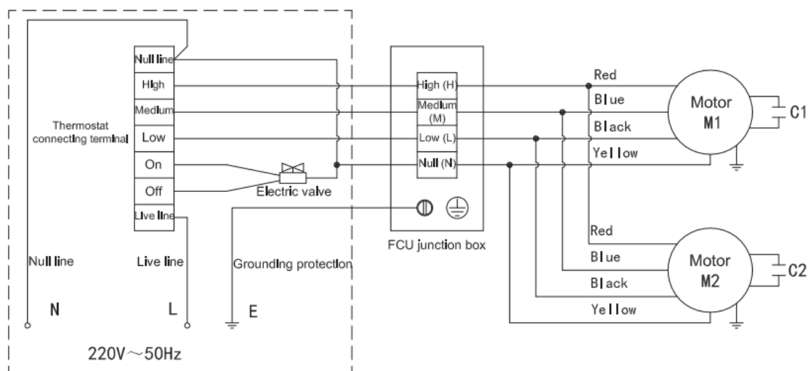
Thermostat (2 Pipes)
