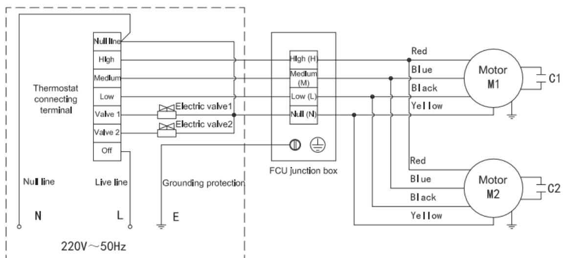
Thermostat (4 Pipes)
